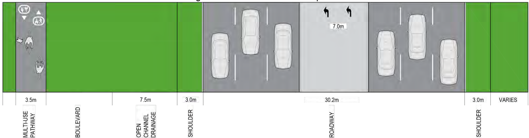
PLAN Lagamodiere Boulevard - Concept-1B & 2B
