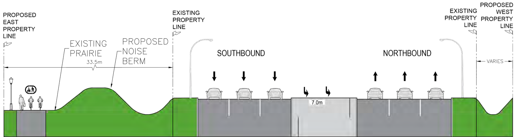
CROSS-SECTION Lagamodiere Boulevard - Concept-1B & 2B
